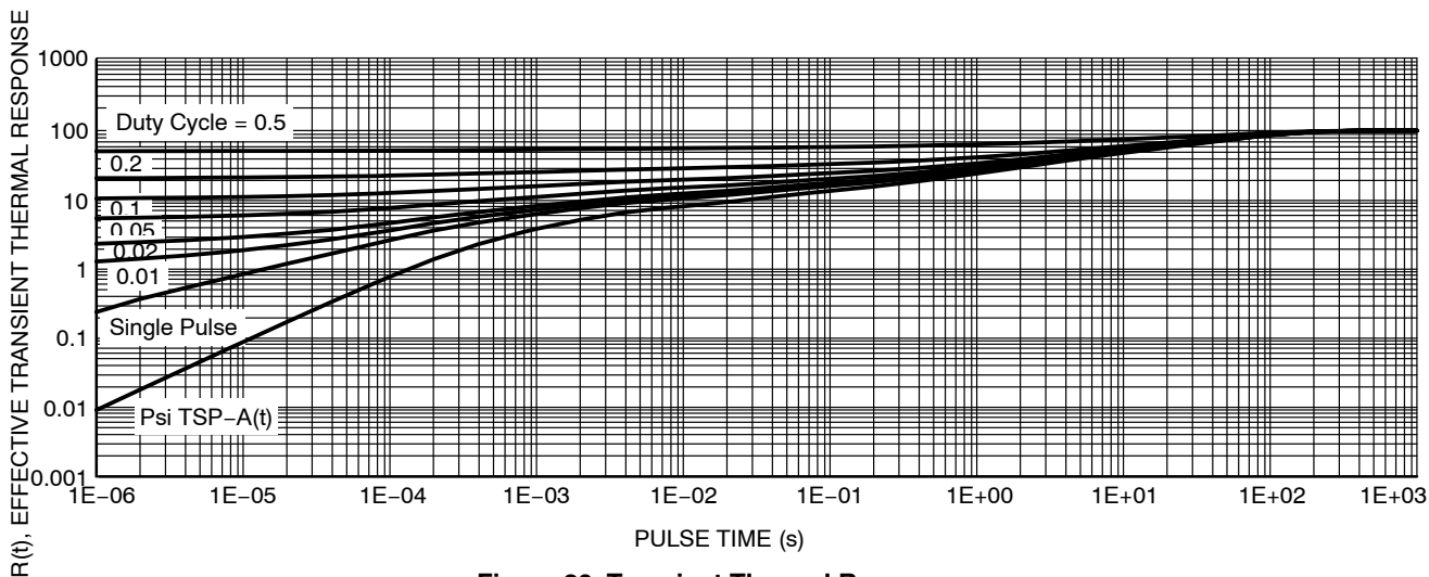
Figure 20. Transient Thermal Response
